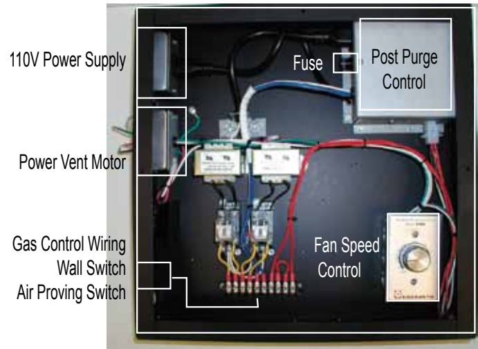
Figure 7. Electrical Supply
